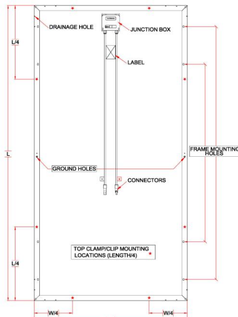
Figure 1 : Module mounting diagram
